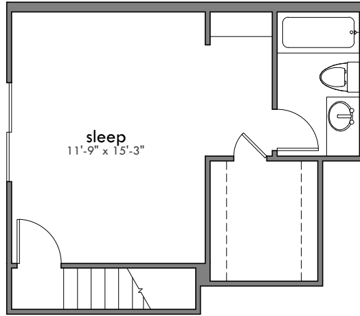
2nd Floor
